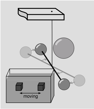
b / A simplified diagram of Kreuzer's modification. The moving teflon mass is submerged in a liquid with nearly the same density.
