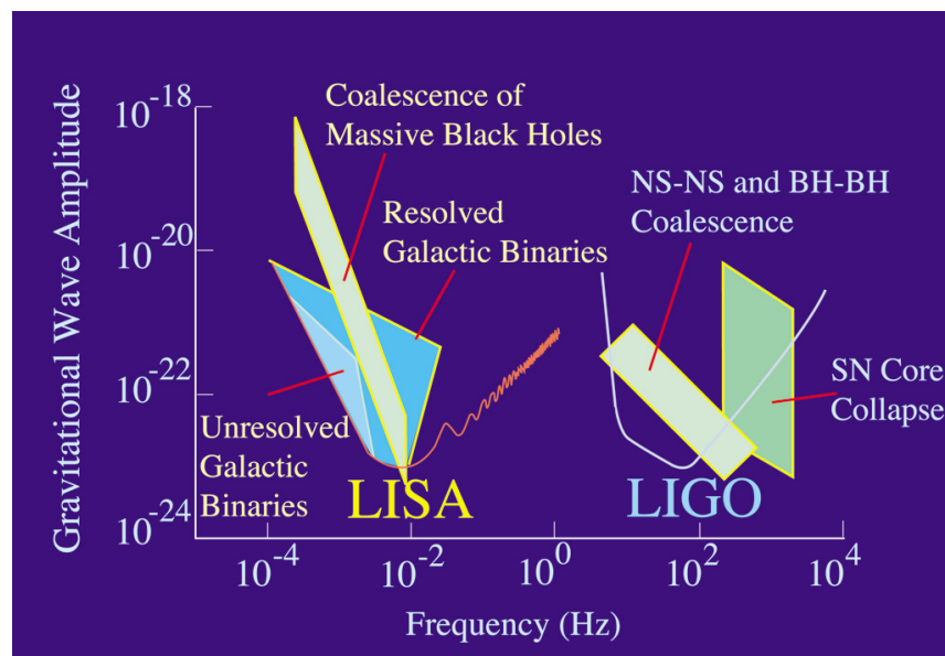
b / Predicted sensitivities of LISA and LIGO to gravitational waves of various frequencies.
