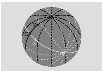
g / Gaussian normal coordinates on a sphere.
