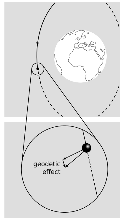
a / The geodetic effect as measured by Gravity Probe B.
