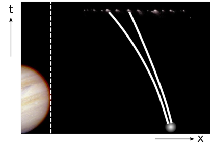
b / Tidal forces cause the initially parallel world-lines of the fragments to diverge. The spacetime occupied by the comet has intrinsic curvature, but it is not caused by any local mass; it is caused by the distant mass of Jupiter.
