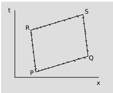
d / Simultaneity is not well defined. The constant-time lines PQ and RS from figure b are not constant-time lines when observed in a different frame of reference.
