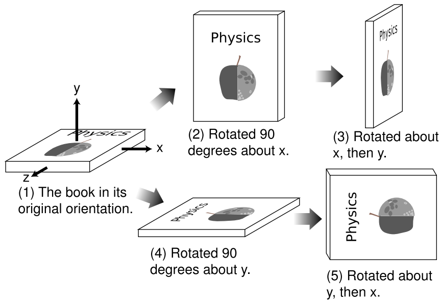
a / Performing the rotations in one order gives one result, 3, while reversing the order gives a different result, 5.
