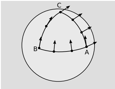
b/ The change in the vector due to parallel transport around the octant equals the integral of the Riemann tensor over the interior.
