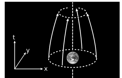
d / A cloud of test masses is released at rest in a spherical shell around the earth, shown here as a circle because the z axis is omitted. The volume of the shell contracts over time, which demonstrates that the local curvature of spacetime is generated by a local source — the earth — rather than some distant one.
