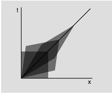
b / A series of Lorentz boosts acts on a square.
