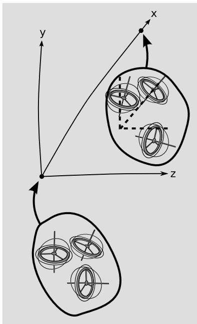
c / Three gyroscopes are initially aligned with the x , y , and z axes. After parallel transport along the geodesic x axis, the x gyroscope is still aligned with the x axis, but the y and z gyroscopes have rotated.
