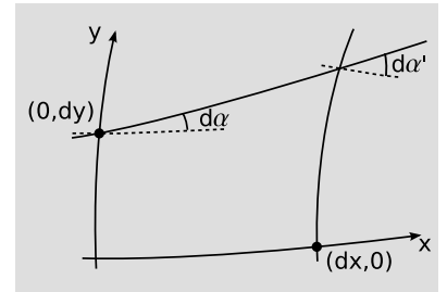
h / 1. Gaussian curvature can be interpreted as the failure of parallelism represented by d^2\alpha/dx dy .
