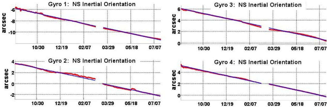
b / Precession angle as a function of time as measured by the four gyroscopes aboard Gravity Probe B.
