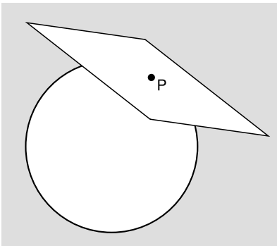
c / The tangent space at a point P on a sphere can be visualized as a Euclidean plane. If coordinates (\theta, \phi) are used, then the partial derivative operators \partial_\theta and \partial_\phi can serve as a basis for the tangent plane.
