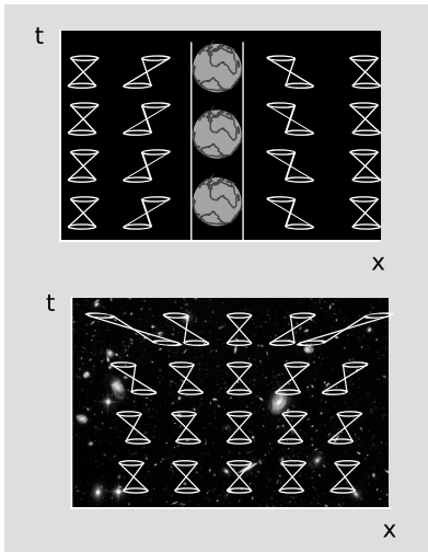
c / Light cones tip over for two reasons in general relativity: because of the presence of masses, which have gravitational fields, and because of the cosmological constant. The time and distance scales in the bottom figure are many orders of magnitude greater than those in the top.
