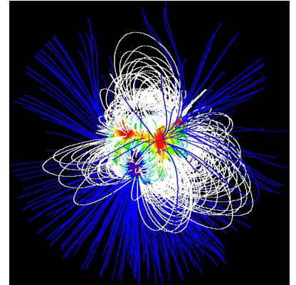
a / Since magnetic field lines can never intersect, a magnetic field pattern contains coordinate-independent information in the form of the knotting of the lines. This figure shows the magnetic field pattern of the star SU Aurigae, as measured by Zeeman-Doppler imaging (Petit et al.). White lines represent magnetic field lines that close upon themselves in the immediate vicinity of the star; blue lines are those that extend out into the interstellar medium.
