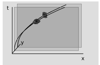
b / Two rocks are dropped side by side. The curvatures of their world-lines are not intrinsic. In a free-falling frame, both would appear straight. If initially parallel world-lines became non-parallel, that would be evidence of intrinsic curvature.
