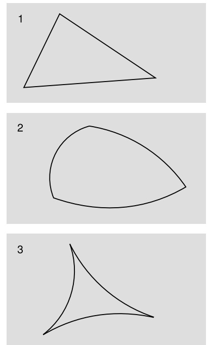
b / 1. In the Euclidean plane, this triangle can be scaled by any factor while remaining similar to itself. 2. In a plane with positive curvature, geometrical figures have a maximum area and maximum linear dimensions. This triangle has almost the maximum area, because the sum of its angles is nearly 3\pi . 3. In a plane with negative curvature, figures have a maximum area but no maximum linear dimensions. This triangle has almost the maximum area, because the sum of its angles is nearly zero. Its vertices, however, can still be separated from one another without limit.
