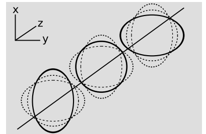
e / As the gravitational wave propagates in the z direction, the metric oscillates in the x and y directions, preserving volume.
