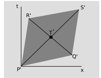
e / Example 5. Flashes of light travel along P'T' and Q'T' . The observer in this frame of reference judges them to have been emitted at different times, and to have traveled different distances.
