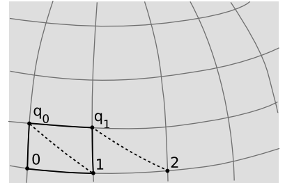
a / Construction of an affine parameter in curved spacetime.
