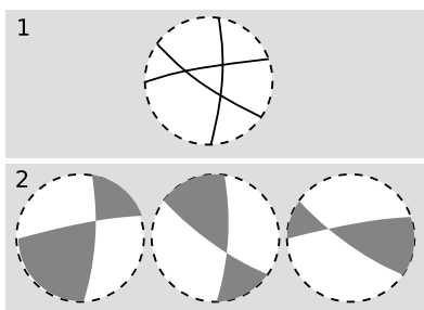
f / Proof that the angular defect of a triangle in elliptic geometry is proportional to its area. Each white circle represents the entire elliptic plane. The dashed line at the edge is not really a boundary; lines that go off the edge simply wrap back around. In the spherical model, the white circle corresponds to one hemisphere, which is identified with the opposite hemisphere.
