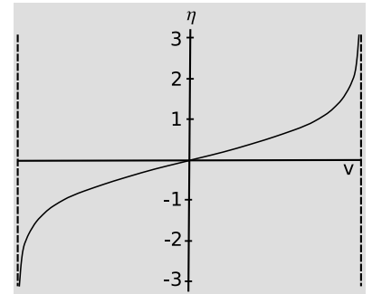
e / The rapidity, \eta = \tanh^{-1} v , as a function of v .
