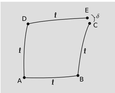
a / Measuring \partial^2 T / \partial x \partial y for a scalar T .
