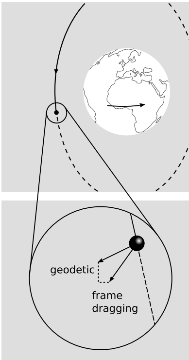
f / Gravity Probe B verified the existence of frame-dragging. The rotational axis of the gyroscope precesses in two perpendicular planes due to the two separate effects: geodetic and frame-dragging.
