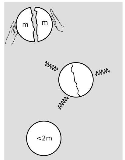
a / The field equations of general relativity are nonlinear.
