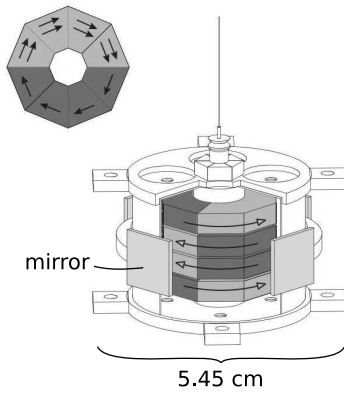
d/The University of Washington torsion pendulum used to search for torsion. The light gray wedges are Alnico, the darker ones \text{SmCo}_5 . The arrows with the filled heads represent the directions of the electron spins, with denser arrows indicating higher polarization. The arrows with the open heads show the direction of the \mathbf{B} field. University of Washington Eot-Wash group, http://www.npl.washington.edu/eotwash/publications/pdf/lowfrontier2.pdf
