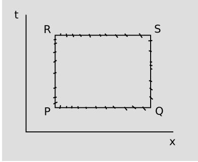
b / Objects are released at rest at spacetime events P and Q. They remain at rest, and their world-lines define a notion of parallelism.
