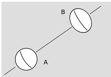
k / One planet rotates about its axis and the other does not. As discussed in more detail on p. 104, Einstein believed that general relativity was even more radically egalitarian about frames of reference than it really is. He thought that if the planets were alone in an otherwise empty universe, there would be no way to tell which planet was really rotating and which was not, so that B's tidal bulge would have to disappear. There would be no way to tell which planet's surface was a Lorentz frame.
