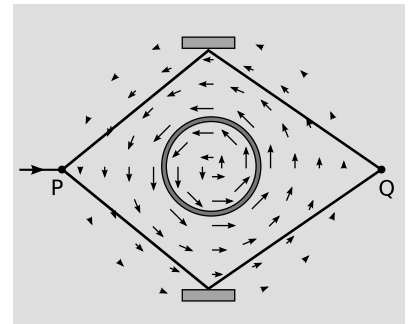
a / The Aharonov-Bohm effect. An electron enters a beam splitter at P, and is sent out in two different directions. The two parts of the wave are reflected so that they reunite at Q. The arrows represent the vector potential A . The observable magnetic field B is zero everywhere outside the solenoid, and yet the interference observed at Q depends on whether the field is turned on. See page 123 for further discussion of the A and B fields of a solenoid.
