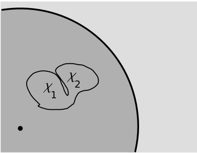
i/ If the crack between the two areas is squashed flat, the two pieces of the path on the interior coincide, and their contributions to the precession cancel out ( \mathbf{v} \rightarrow -\mathbf{v} , but \mathbf{a} \rightarrow +\mathbf{a} , so \mathbf{a} \times \mathbf{v} \rightarrow -\mathbf{a} \times \mathbf{v} ). Therefore the precession \chi obtained by going around the outside is equal to the sum \chi_1 + \chi_2 of the precessions that would have been obtained by going around the two parts.
