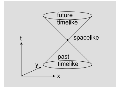
a / The light cone in 2+1 dimensions.
