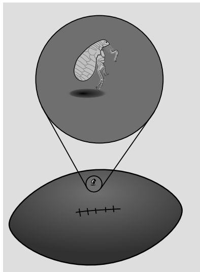
k / A flea on the football cannot orient himself by intrinsic, local measurements.
