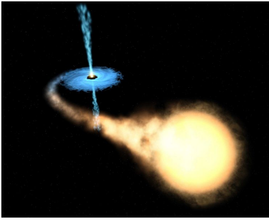
a / A black hole accretes matter from a companion star.
