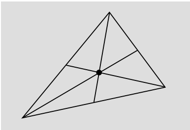
f / Affine geometry gives a well-defined centroid for the triangle.
