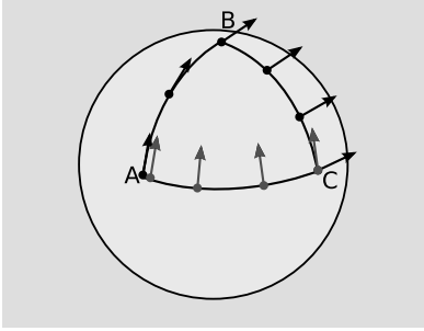
b / Parallel transport is path-dependent. On the surface of this sphere, parallel-transporting a vector along ABC gives a different answer than transporting it along AC.
