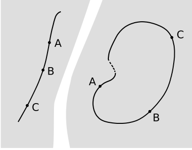
a / Axioms O2 (left) and O3 (right).
