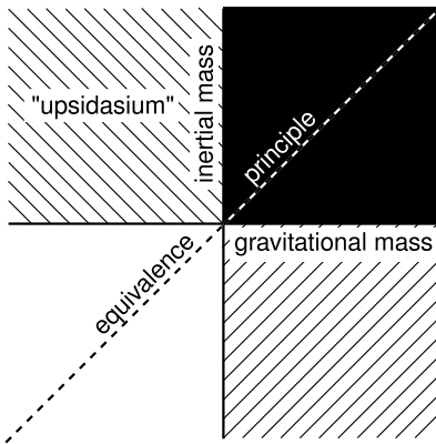
e / Negative mass.
