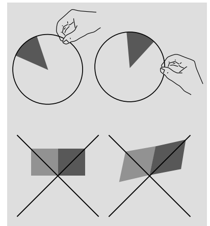
b / The circle plays a privileged role in Euclidean geometry. When rotated, it stays the same. The pie slice is not invariant as the circle is. A similar privileged place is occupied by the light cone in Lorentz geometry. Under a Lorentz boost, the spacetime parallelograms change, but the light cone doesn't.
