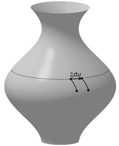
a / The two-dimensional space has a symmetry which can be visualized by imagining it as a surface of revolution embedded in three-space. Without reference to any extrinsic features such as coordinates or embedding, an observer on this surface can detect the symmetry, because there exists a vector field \xi du such that translation by \xi du doesn't change the distance between nearby points.
