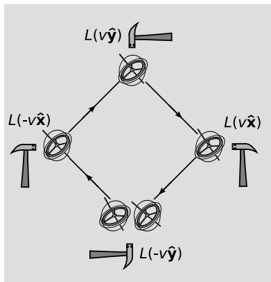
c / Classically, the gyroscope should not rotate as long as the forces from the hammer are all transmitted to it at its center of mass.
