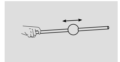
d / The sticky bead argument for the reality of gravitational waves. As a gravitational wave with the appropriate polarization passes by, the bead vibrates back and forth on the rod. Friction creates heat. This demonstrates that gravitational waves carry energy, and are thus real, observable phenomena.
