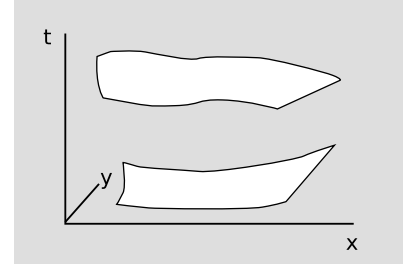
a / Two spacelike surfaces.
