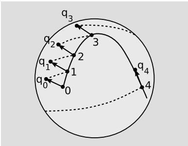
c / Bad things happen if we try to construct an affine parameter along a curve that isn't a geodesic. This curve is similar to path ABC in figure b. Parallel transport doesn't preserve the vectors' angle relative to the curve, as it would with a geodesic. The errors in the construction blow up in a way that wouldn't happen if the curve had been a geodesic. The fourth dashed parallel flies off wildly around the back of the sphere, wrapping around and meeting the curve at a point, 4, that is essentially random.
