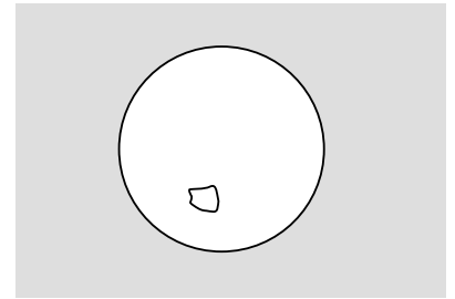
b / We define a boundary around a region whose charge we want to measure.
