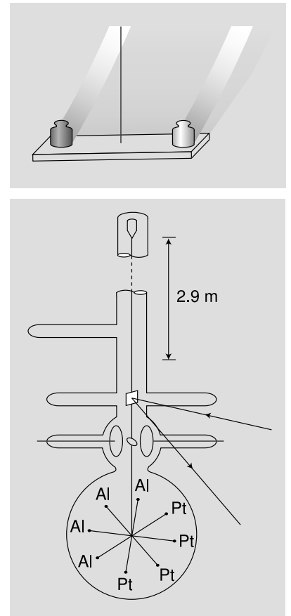
e / An Eötvös experiment. Top: simplified version. Bottom: realistic version by Braginskii and Panov. (Drawing after Braginskii and Panov.)
