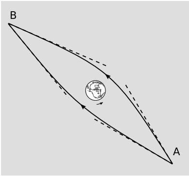
e / Two light rays travel in the earth's equatorial plane from A to B. Due to frame-dragging, the ray moving with the earth's rotation is deflected by a greater amount than the one moving contrary to it. As a result, the figure has an asymmetric banana shape. Both the deflection and its asymmetry are greatly exaggerated.
