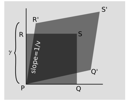
c / Unit square PQRS is Lorentz-boosted to the parallelogram P'Q'R'S'.
