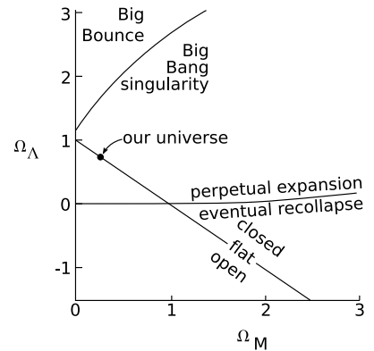
f / The cosmological parameters of our universe, after Perlmutter et al., arxiv.org/abs/astro-ph/9812133 .
