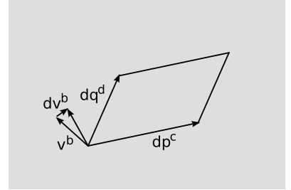
a / The definition of the Riemann tensor. The vector v^b changes by dv^b when parallel-transported around the approximate parallelogram. ( v^b is drawn on a scale that makes its length comparable to the infinitesimals dp^c , dq^d , and dv^b ; in reality, its size would be greater than theirs by an infinite factor.)
