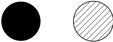
f / The black sphere is made of ordinary matter. The crosshatched sphere has positive gravitational mass and negative inertial mass. If the two of them are placed side by side in empty space, they will both accelerate steadily to the right, gradually approaching the speed of light. Conservation of momentum is preserved, because the exotic sphere has leftward momentum when it moves to the right, so the total momentum is always zero.
