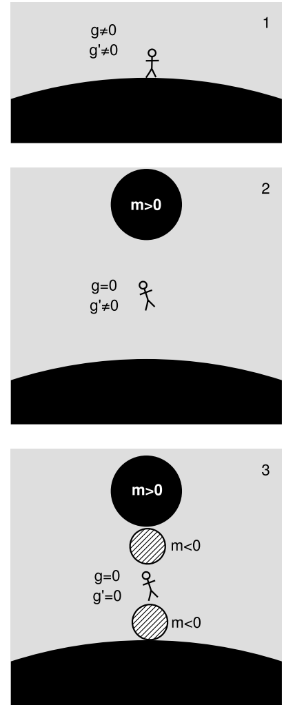
g / Nulling out a gravitational field is impossible in one dimension without exotic matter. 1. The planet imposes a nonvanishing gravitational field with a nonvanishing gradient. 2. We can null the field at one point in space, by placing a sphere of very dense, but otherwise normal, matter overhead. The stick figure still experiences a tidal force, g' \neq 0 . 3. To change the field’s derivative without changing the field, we can place two additional masses above and below the given point. But to change its derivative in the desired direction — toward zero — we would have to make these masses negative.
