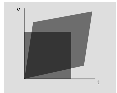
a / Two objects at rest have world-lines that define a rectangle. In a second frame of reference in motion relative to the first one, the rectangle becomes a parallelogram.
