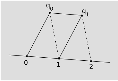
e / Construction of an affine parameter.
