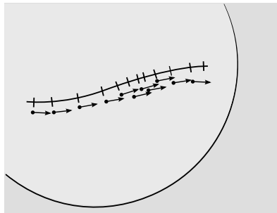
a / The tick marks on the line define a coordinate measured along the line. It is not possible to set up such a coordinate system globally so that the coordinate is uniform everywhere. The arrows represent changes in the value coordinate; since the changes in the coordinate are all equal, the arrows are all the same length.
