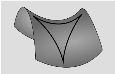
j / A triangle in a space with negative curvature has angles that add to less than \pi .
