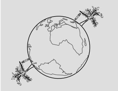
j / Two local Lorentz frames.
