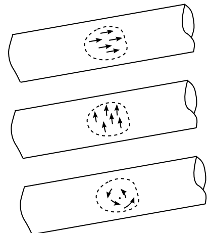
d / Example 3: A cylinder has three local symmetries, but only two that can be extended globally to make Killing vectors.
