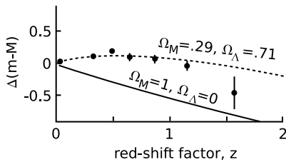
e / A Hubble plot for distant supernovae. Each data point represents an average over several different supernovae with nearly the same z .
