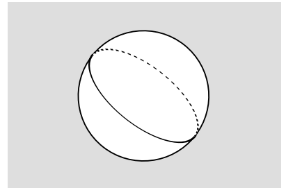
c / This boundary cuts the sphere into equal parts.
