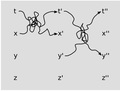
a / A boost along x followed by a boost along y results in tangling up of the x and y coordinates, so the result is not just a boost but a boost plus a rotation.
