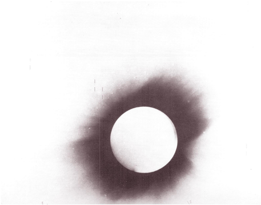
c / One of the photos from Eddington's observations of the 1919 eclipse. This is a photographic negative, so the circle that appears bright is actually the dark face of the moon, and the dark area is really the bright corona of the sun. The stars, marked by lines above and below them, appeared at positions slightly different than their normal ones, indicating that their light had been bent by the sun's gravity on its way to our planet.
