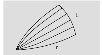
i / 2. Gaussian curvature as L \neq r\theta .
