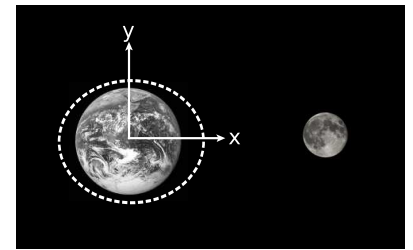
c / The moon's gravitational field causes the Earth's oceans to be distorted into an ellipsoid. The sign of the sectional curvature is negative in the x - t plane, but positive in the y - t plane.
