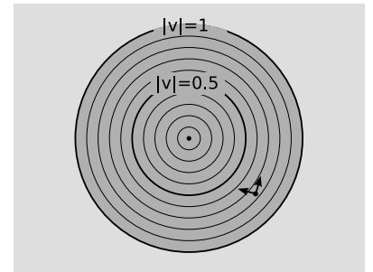
e / The velocity disk.
