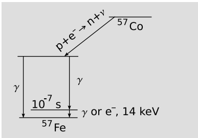
o / The Pound-Rebka experiment.
