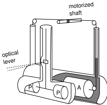
c / The Kreuzer experiment. 1. There are two passive masses, P, and an active mass A consisting of a single 23-cm diameter teflon cylinder immersed in a fluid. The teflon cylinder is driven back and forth with a period of 400 s. The resulting deflection of the torsion beam is monitored by an optical lever and canceled actively by electrostatic forces from capacitor plates (not shown). The voltage required for this active cancellation is a measure of the torque exerted by A on the torsion beam. 2. Active mass as a function of temperature. 3. Passive mass as a function of temperature. In both 2 and 3, temperature is measured in units of ohms, i.e., the uncalibrated units of a thermistor that was immersed in the liquid.
