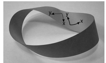
a / A Möbius strip is not an orientable surface.
