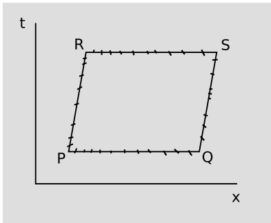
c / There is no well-defined angular measure in this geometry. In a different frame of reference, the angles are not right angles.
