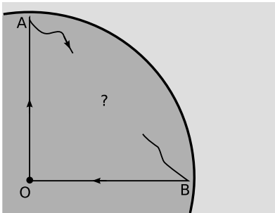
g / A round-trip involving ultrarelativistic velocities. All three legs are at constant acceleration.
