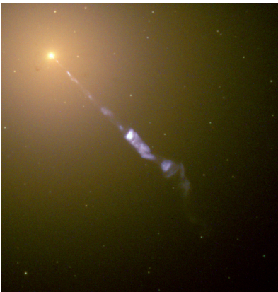
d / A relativistic jet.
