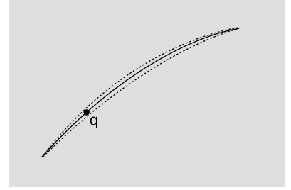
c / The charged particle follows a trajectory that extremizes \int f_b dx^b compared to other nearby trajectories. Relativistically, the trajectory should be understood as a world-line in 3+1-dimensional spacetime.
