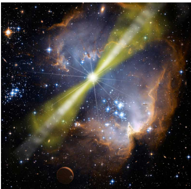
a / An artist's conception of a gamma-ray burst, resulting from a supernova explosion.
