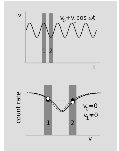
q / Top : A graph of velocity versus time for the source. The velocity has both a constant component and an oscillating one with a frequency of 10-50 Hz. The constant component v_0 was used as a way of determining the calibration of frequency shift as a function of count rates. Data were acquired during the quarter-cycle periods of maximum oscillatory velocity, 1 and 2. Bottom : Count rates as a function of velocity, for v_0 = 0 and v_1 \neq 0 . The dashed curve and black circles represent the count rates that would have been observed if there were no gravitational effect. The gravitational effect shifts the resonance curve to one side (solid curve), resulting in an asymmetry of the count rates (open circles). The shift, and the resulting asymmetry, are greatly exaggerated for readability; in reality, the gravitational effect was 500 times smaller than the width of the resonance curve.
