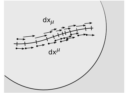
b / The vectors dx^\mu and dx_\mu are duals of each other.
