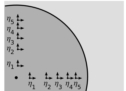
f / Two excursions in a rocket-ship: one along the y axis and one along x .
