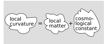
a / The expected structure of the field equations in general relativity.
