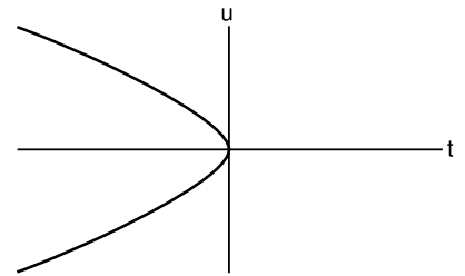
a / The change of coordinates is degenerate at t = 0 .
