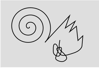
a / This curve has no intrinsic curvature.
