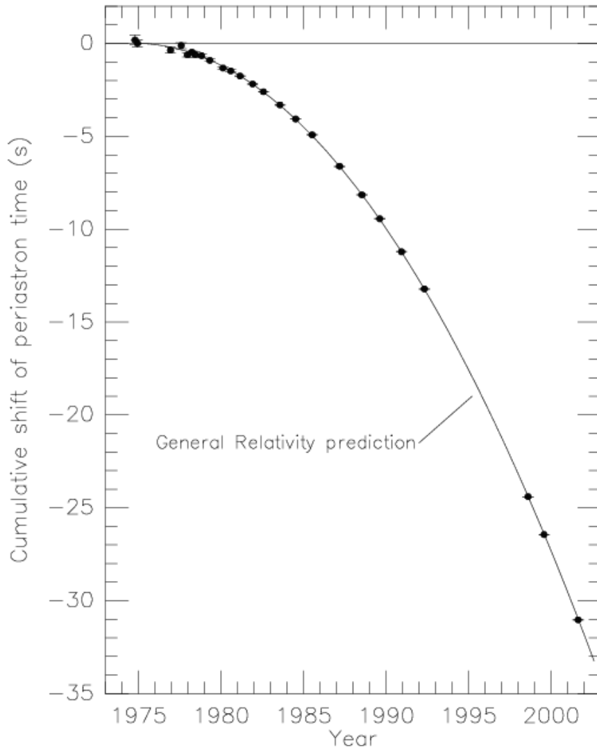
a / The Hulse-Taylor pulsar's orbital motion is gradually losing energy due to the emission of gravitational waves. The linear decrease of the period is integrated on this plot, resulting in a parabola. From Weisberg and Taylor, http://arxiv.org/abs/astro-ph/0211217 .
