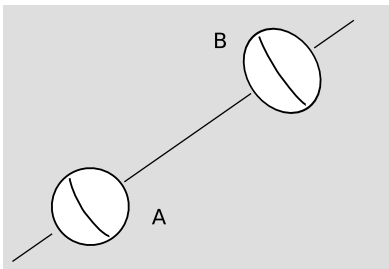
b / A paradox? Planet A has no equatorial bulge, but B does. What cause produces this effect? Einstein reasoned that the cause couldn’t be B’s rotation, because each planet rotates relative to the other.
