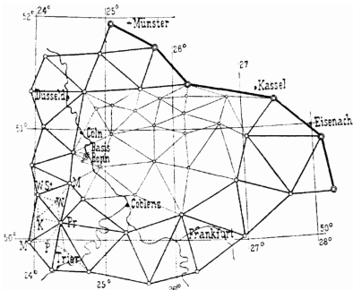
c / A map of a triangulation survey such as the one Gauss carried out. By measuring the interior angles of the triangles, one can determine not just the two-dimensional projection of the grid but its complete three-dimensional form, including both the curvature of the earth (note the curvature of the lines of latitude) and the height of features above and below sea level.
