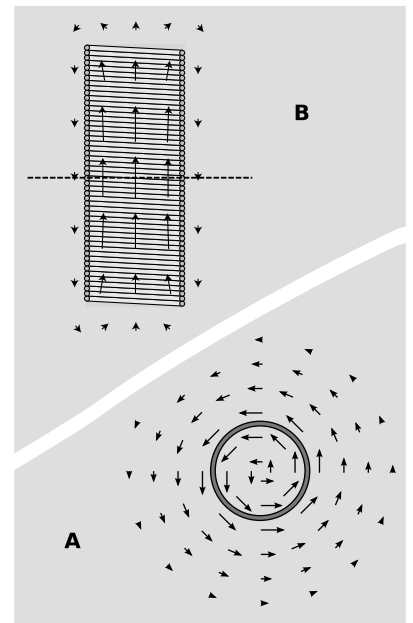
d / The magnetic field (top) and vector potential (bottom) of a solenoid. The lower diagram is in the plane cutting through the waist of the solenoid, as indicated by the dashed line in the upper diagram. For an infinite solenoid, the magnetic field is uniform on the inside and zero on the outside, while the vector potential is proportional to r on the inside and to 1/r on the outside.
