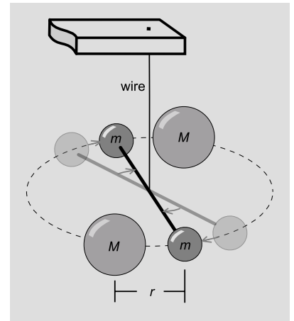
a / A Cavendish balance, used to determine the gravitational constant.
