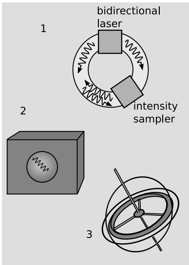
b / Inertial devices for maintaining a direction in space: 1. A ring laser. 2. The photon in a perfectly reflective spherical cavity. 3. A gyroscope.
