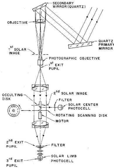
a / The apparatus used by Dicke and Goldenberg to measure the oblateness of the sun was essentially a telescope with a disk inserted in order to black out most of the light from the sun.
