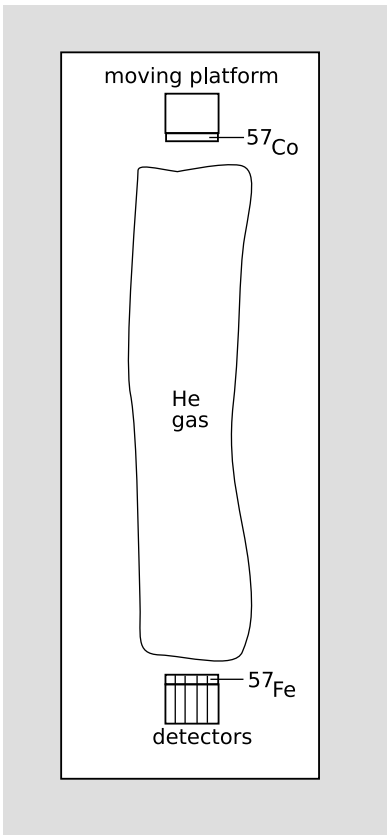
o / The Pound-Rebka experiment.
